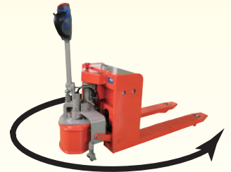
Minimum Turning Radius: 1620mm
