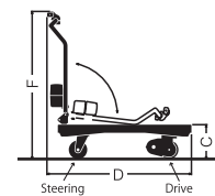
■ Dimensions(ASP-300-T3)
