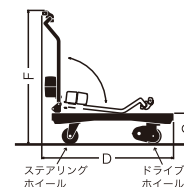
■寸法図(ASP-300-T3)
