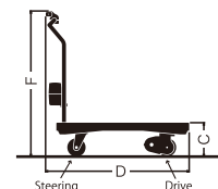
■ Dimensions(ASP-300-T2)
